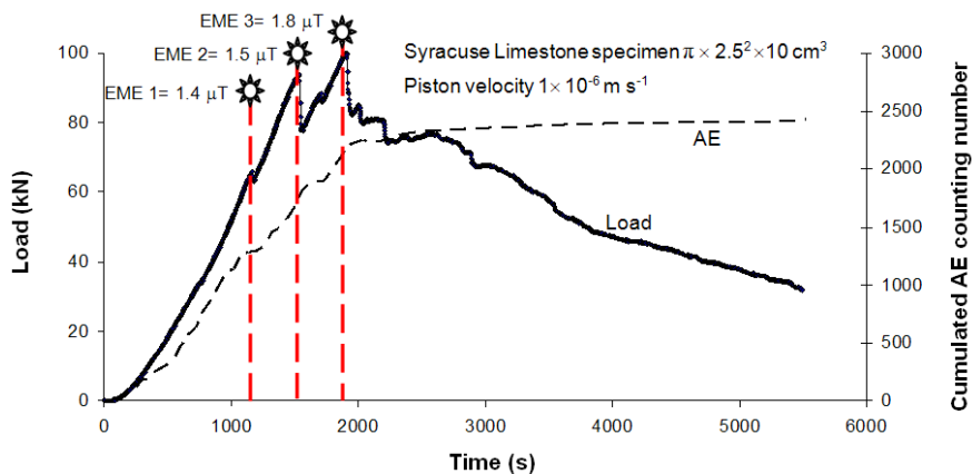
Figure 4: Load vs. time curve of the Syracuse Limestone specimen (bold line). The dashed line represents the cumulated number of AE. The stars on the graph show the moments of EME events with magnetic fields comprised between 1.4 and 1.8 \mu T.
