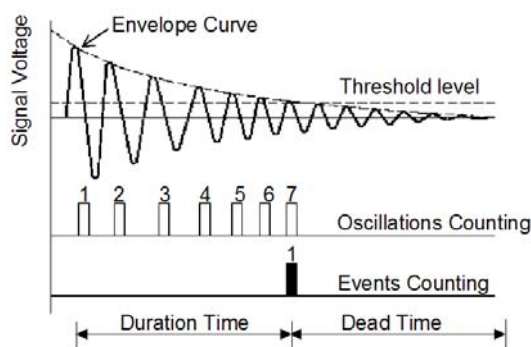
Figure 1: Schematic signal detected by AE technique
