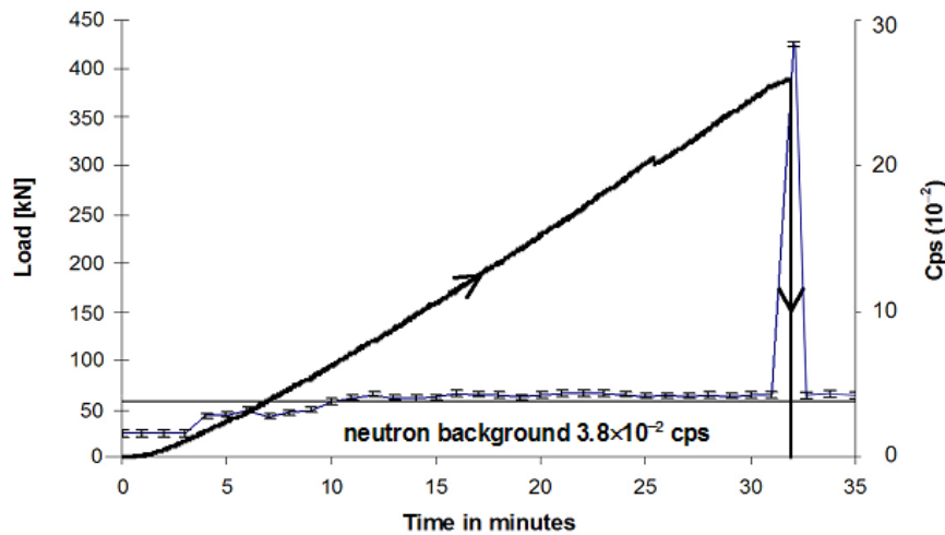
Figure 5: Load vs. time and cps curves for one of the test specimens in Luserna Granite.
