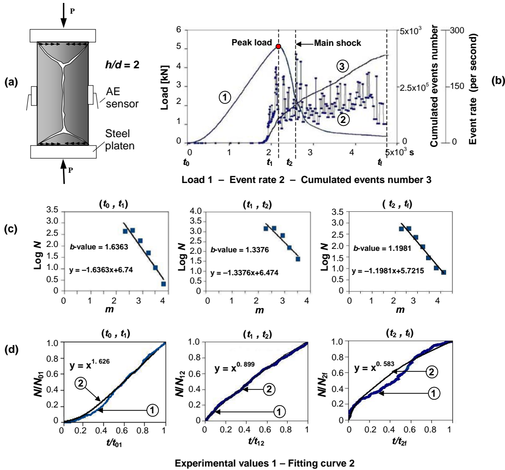
Figure 3: Cylindrical concrete specimen in compression. (a) Testing set-up. (b) Load vs. time curve and AE activity. (c) b -values during the test. (d) Variation in \beta_t parameter during the test.
