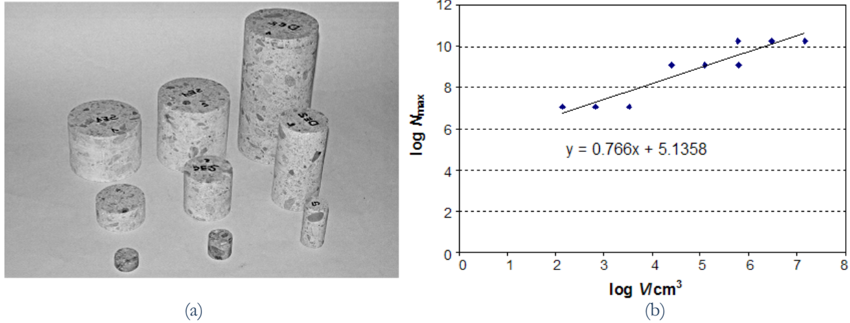
Figure 2: (a) Geometries of the tested specimens. (b) Volume-effect on N_{\max} .
