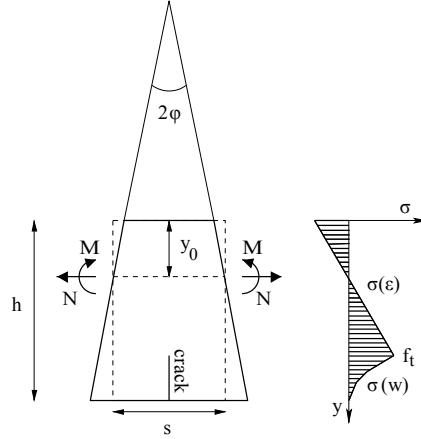
Figure 2. The hinge model and assumed stress distribution.
