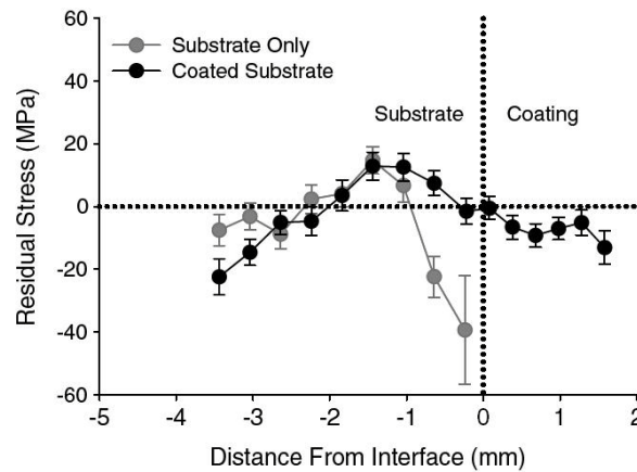
Figure 13: Residual stress measurement of CS Al coating [60].
