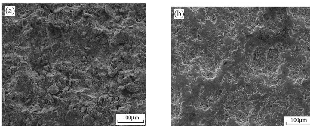
Figure 12: Surface morphology of as-sprayed NiCrAlY bond coating (a) and after shot-peened NiCrAlY bond coating (b)[58].
