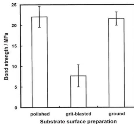
Figure 9: Bar chart showing the effect of substrate condition on the bond strength of deposits sprayed at 29 bar gas pressure using CTi powder(course powder) (error bars represent the standard error of the mean)[55].
