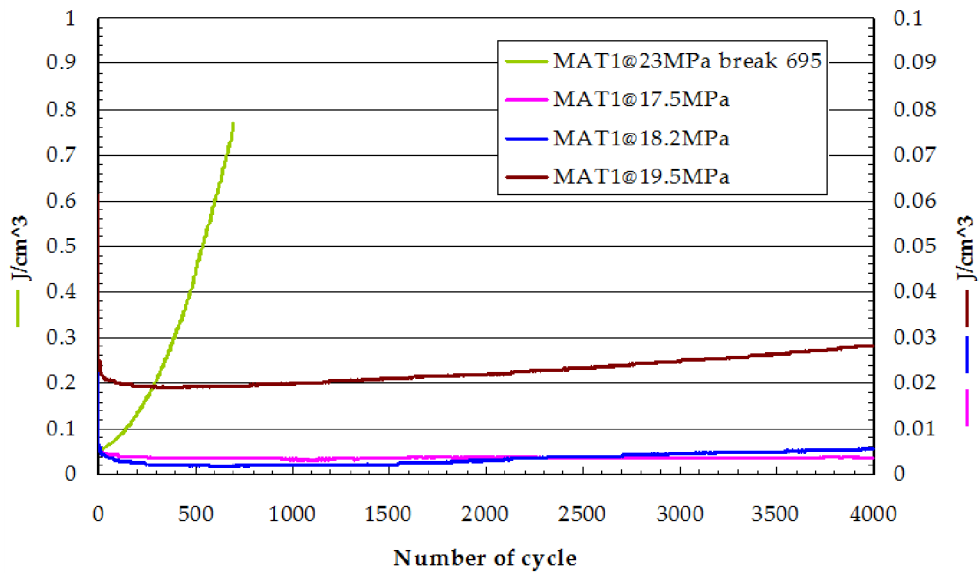
Figure 3: dissipated strain energy for MAT1.
