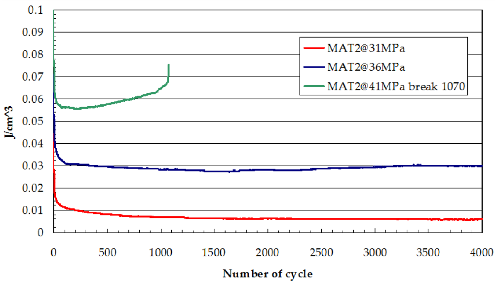
Figure 6: dissipated strain energy for MAT2.
