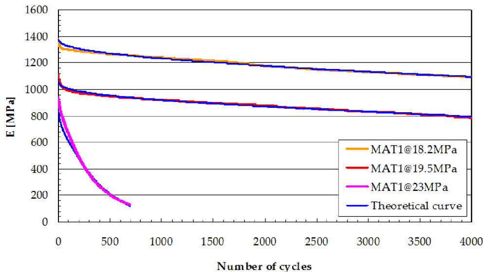
Figure 13: MAT1 Secant Modulus drop fitted by Tao model.
