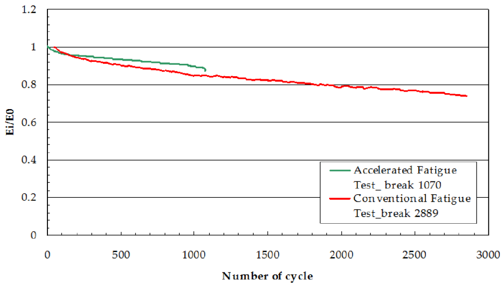
Figure 8: comparison between conventional and accelerated fatigue test on MAT2.
