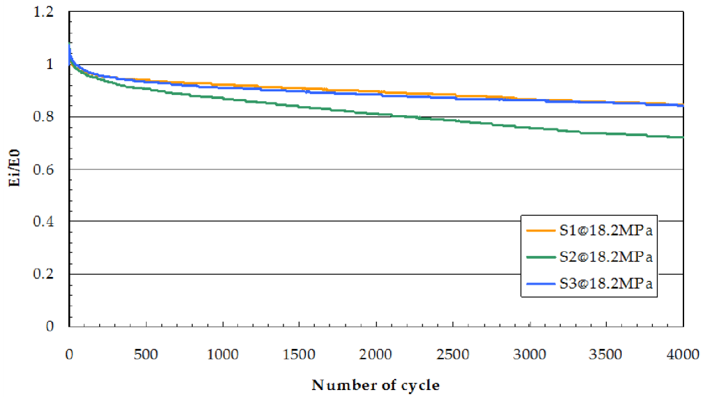
Figure 10: comparison between S1, S2, S3 secant modulus drop.
