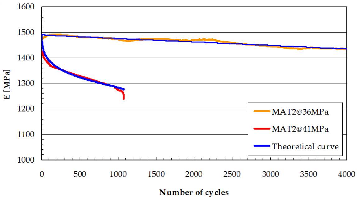
Figure 14: MAT2 Secant Modulus drop fitted by Tao model.
