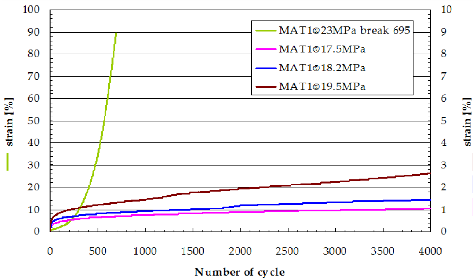
Figure 4: residual strain for MAT1.
