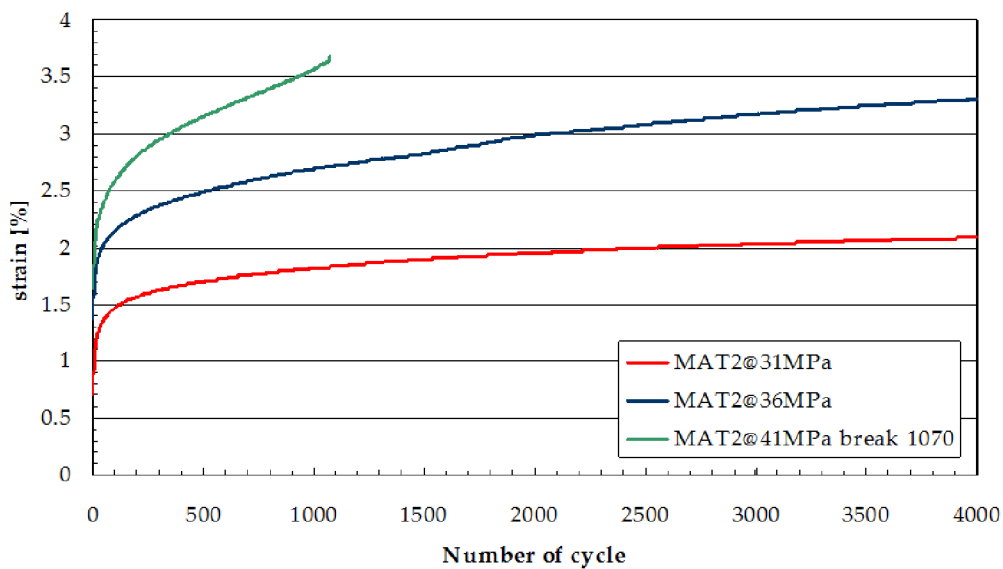
Figure 7: residual deformation for MAT2.
