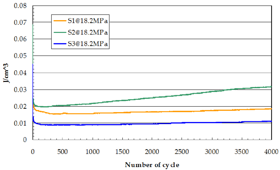
Figure 11: comparison between S1, S2, S3 dissipated strain energy.
