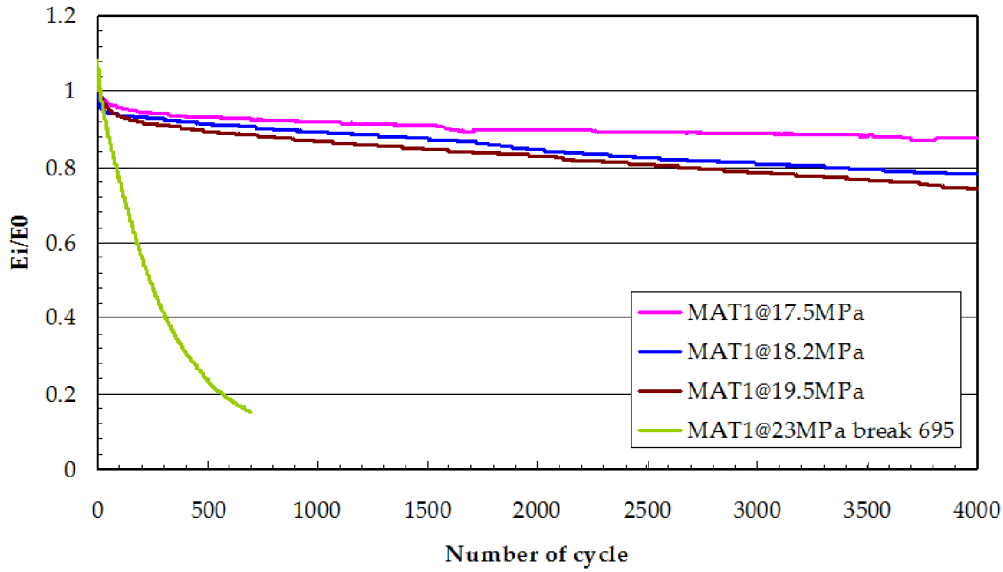
Figure 2: relative secant modulus for MAT1.
