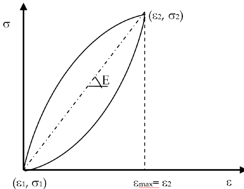
Figure 1: Secant Modulus E as slope of the hysteresis loop.
