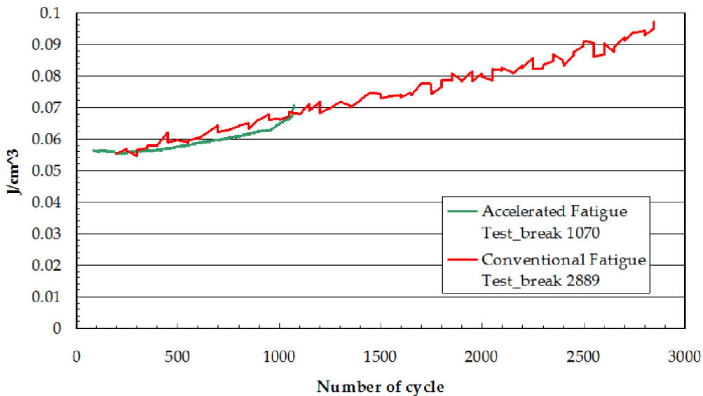
Figure 9: comparison between conventional and accelerated fatigue test on MAT2.
