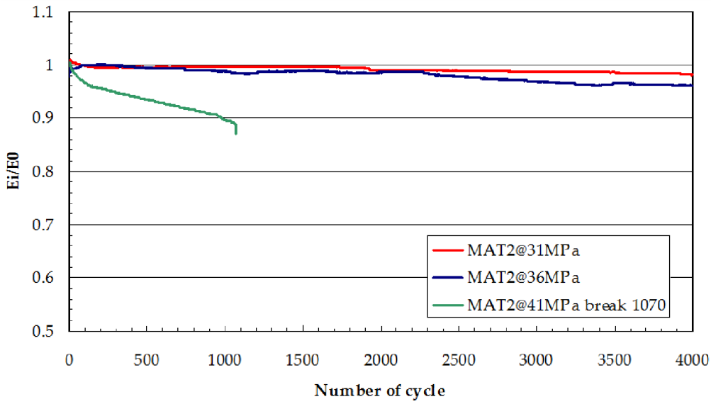
Figure 5: relative secant modulus for MAT2.
