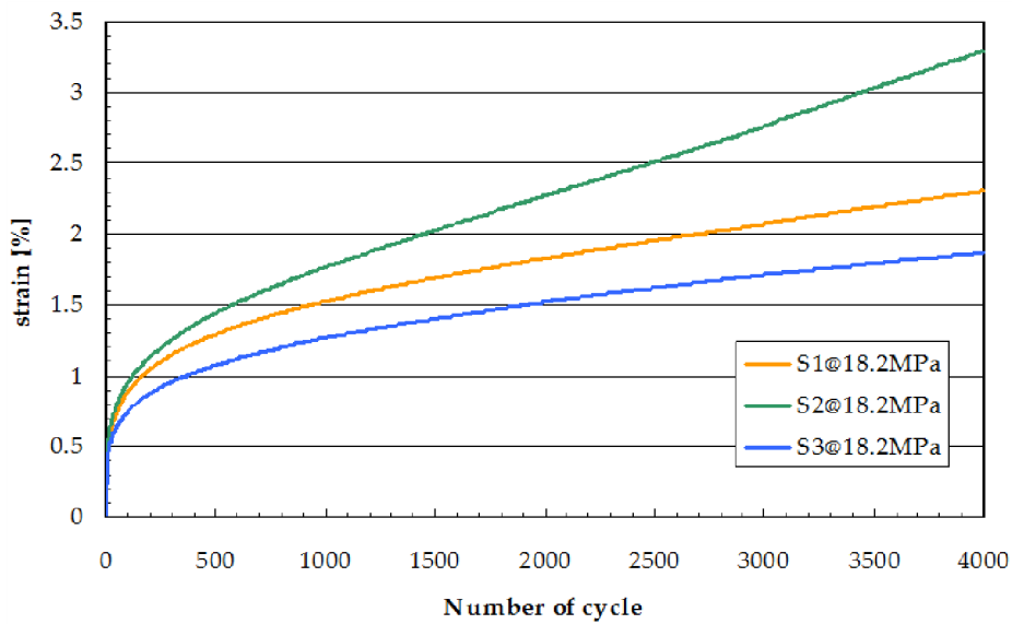
Figure 12: comparison between S1, S2, S3 residual deformation.
