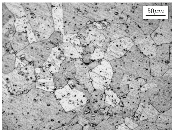
Figure 1: Microstructure of the as-received Haynes 230 material showing twins and a wide range of grain sizes, together with a large number of carbides.
